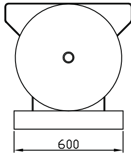
450 Litre HORIZONTAL TANKS WITH BASE PLATES
