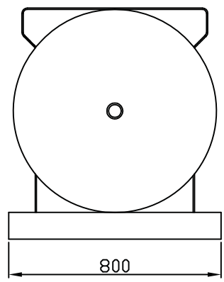
800 Litre HORIZONTAL TANKS WITH BASE PLATES
